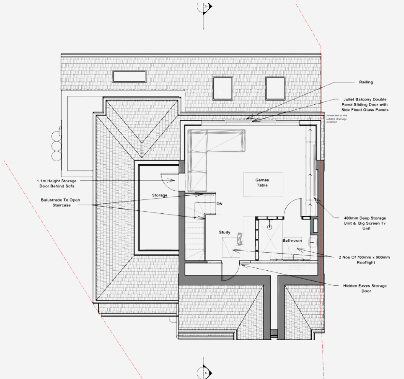
Proposed Loft
